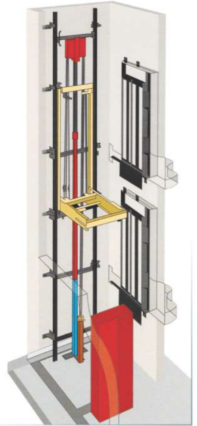
Hydraulic Elevator (Rope Type)
