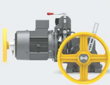
M67 Geared Traction Machine
